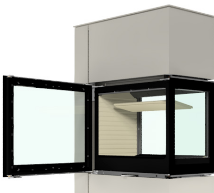
Remove the upper smoke deflector plate
